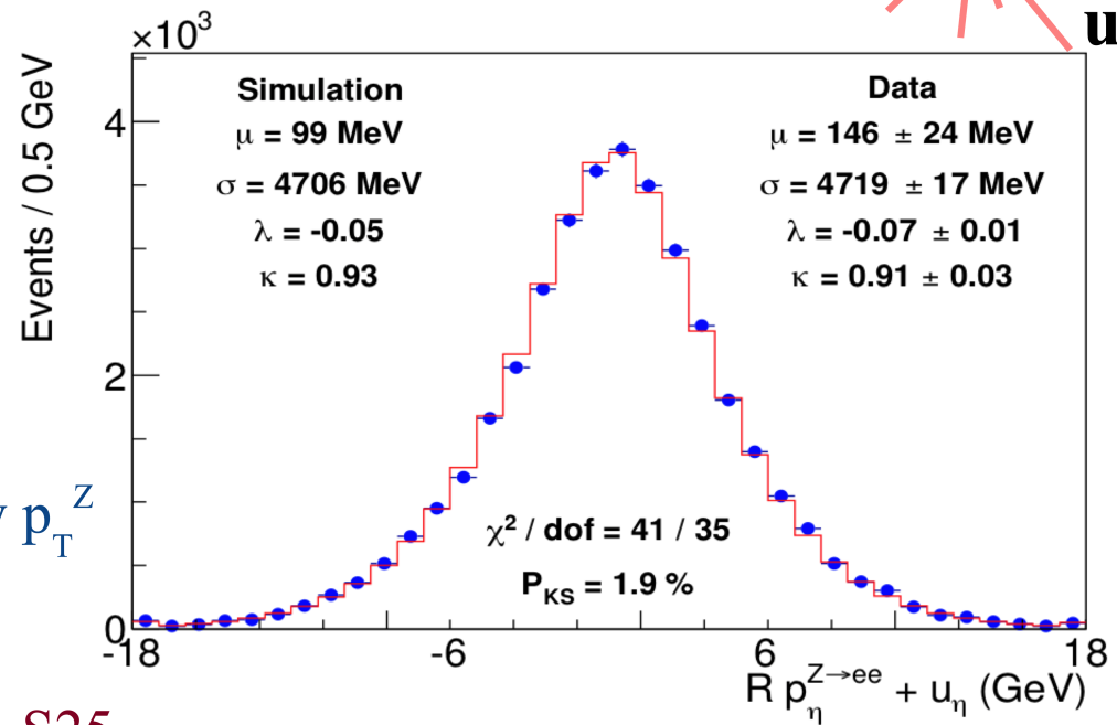
low p_T^Z
