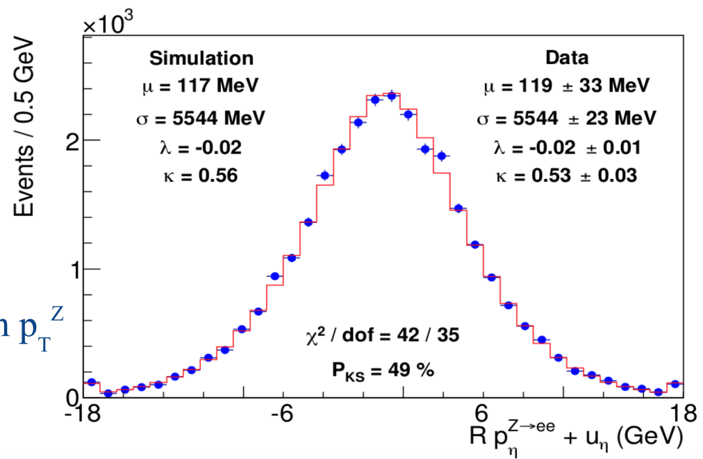
low p_T^Z
