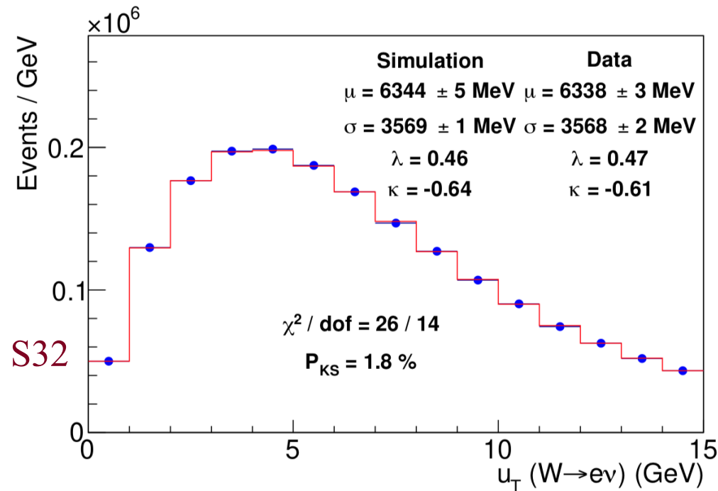
p_T(W) , electron channel
