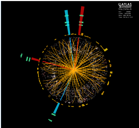
5 Caption: Detection of a Higgs boson event by the ATLAS experiment operating at the LHC in 2012. Credit CERN.
