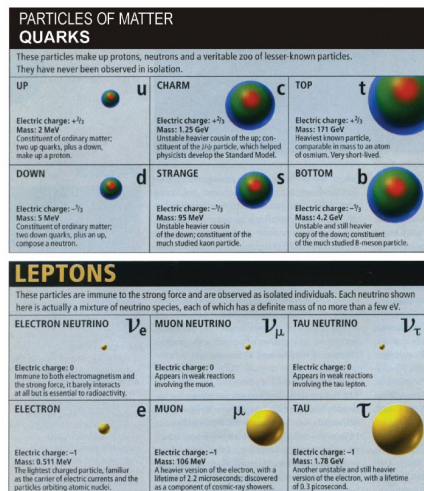
1 Caption: Fundamental particles of matter depicted pictorially: Quarks and Leptons.
