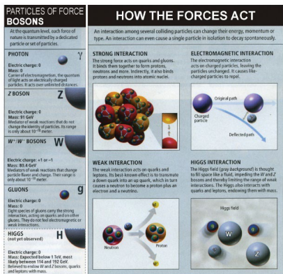
2 Caption: Fundamental particles of matter. Force carrying bosons and their interaction with matter particles.
