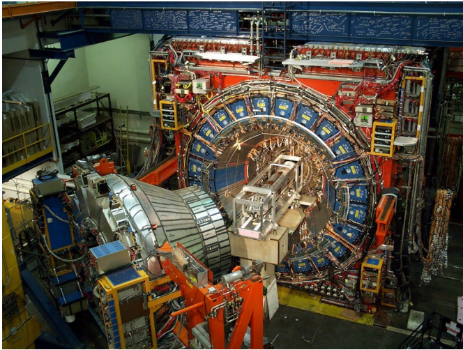
4 Caption: Installation of the CDF experiment at Fermilab. Credit: Fermilab.
