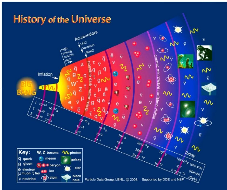
3 Caption: Origin and evolution of the Universe.
