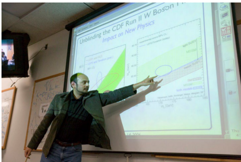
7 Caption: Ashutosh unveiling the W boson mass measurement to colleagues on December 14, 2006. Credit: Fermilab.
