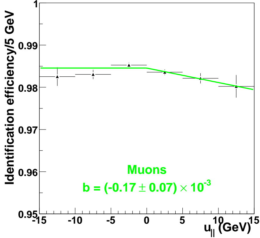
FIGURE 7.2: Variation of the muon identification efficiency as a function of u_{\parallel} , the recoil component in the direction of the muon.
