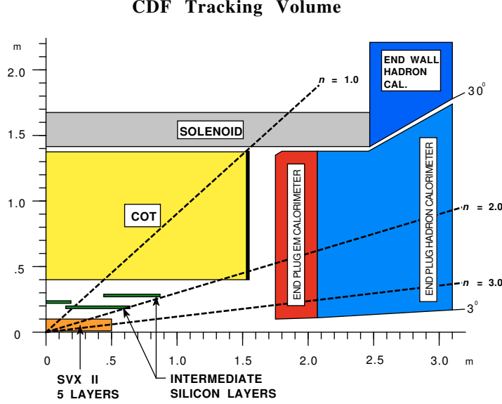
FIGURE 3.2: A schematic view of the \eta coverage of the CDF tracking system.
