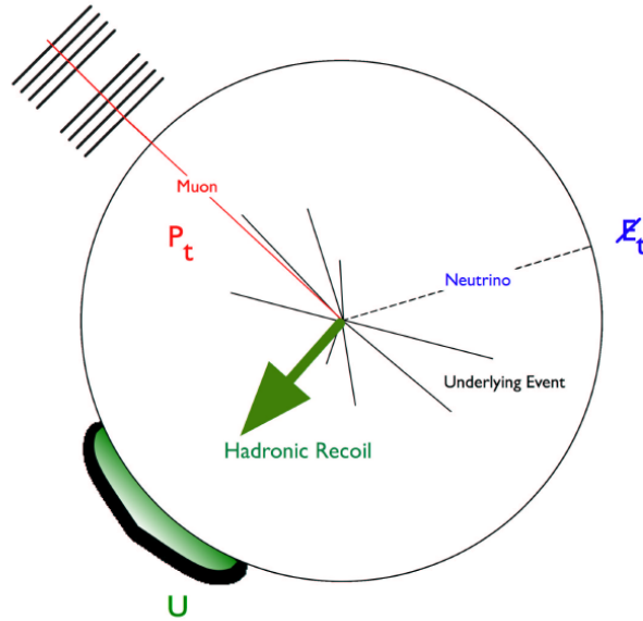
FIGURE 4.2: Axial view of a W \rightarrow \mu\nu event in the CDF detector. The hadronic recoil deposits energy in calorimeter, the muon track leaves hits in the muon chambers and the neutrino escapes detection [59].
