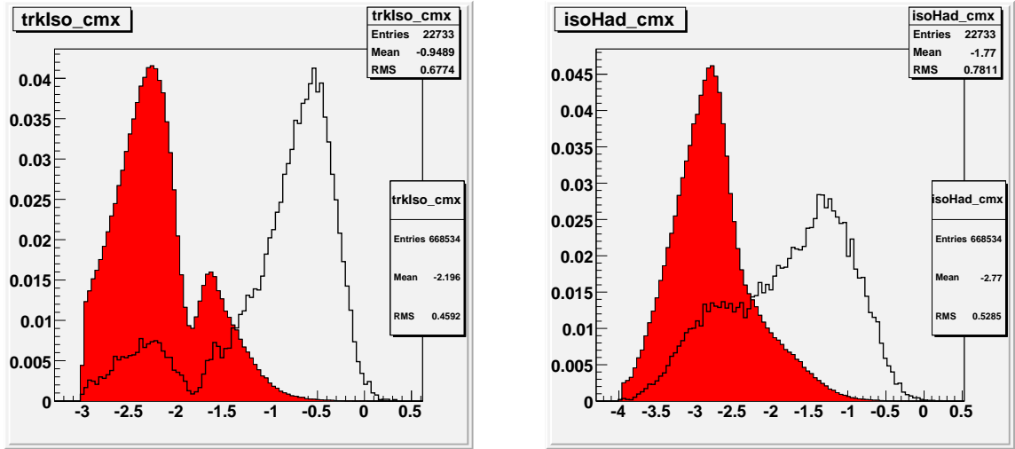
FIGURE H.2: The log distributions of trkIso (left) and hadIso (right) for Z muons of CMX type. The red histogram is for Z MC muon while the black histogram is for QCD jet events from W boson candidates with p_T^\nu < 10 GeV and u_T < 45 GeV.
