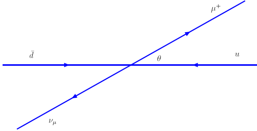
FIGURE 4.3: W^+ decay in the center of mass frame.
