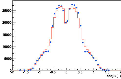
FIGURE 8.26: Data and simulation distributions of \cot \theta of the decay muons.
