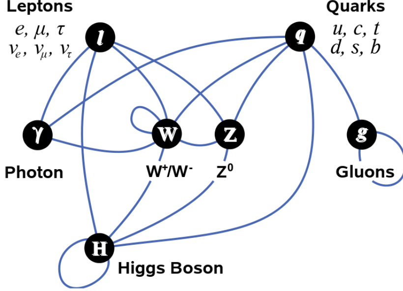
FIGURE 1.2: Summary of particle interactions described by the SM, assuming the Higgs boson exists.
