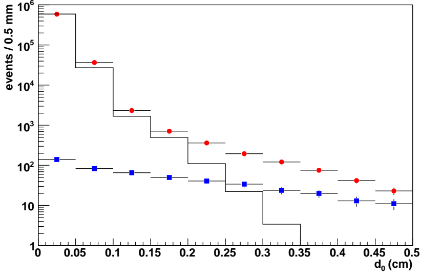
FIGURE 9.1: Comparison of the impact parameter d_0 distributions. The red points are for the W boson candidate sample, the black histogram is for W boson simulation from DukeSim, and the blue points are for a DIF-enriched data sample obtained by anti-selecting on the N_{\text{trans}} . We use 0.2 < d < 0.5 cm to obtain DIF sample.
