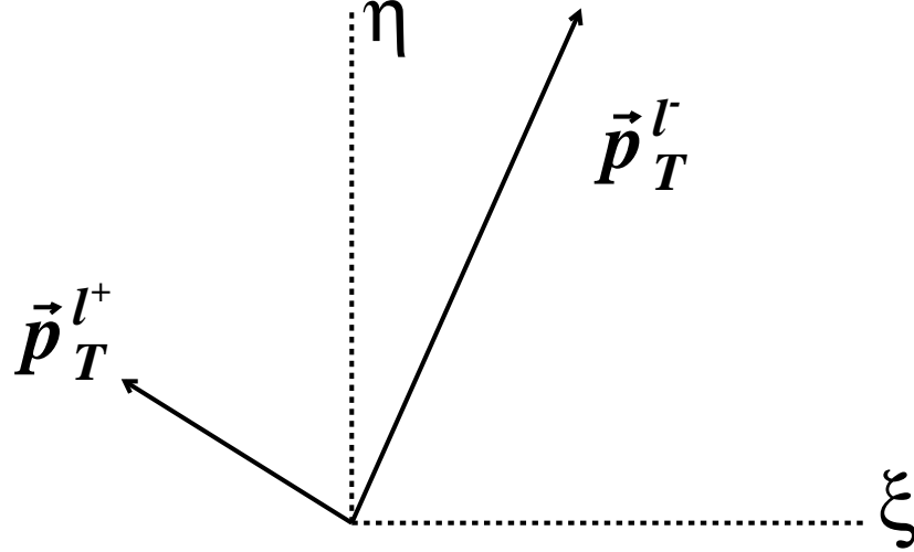
FIGURE 10.3: The \vec{p}_T vectors of the two leptons in Z \rightarrow l^+l^- events. The \eta axis is parallel to the \vec{p}_T(l\bar{l}) direction and the \xi axis is perpendicular to it.
