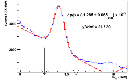
FIGURE F.8: Fitted \Delta p/p of the eighth \langle 1/p_T^\mu \rangle bin in Figure 8.18.
