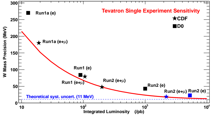
FIGURE 12.3: Projection of measurement precision of the W boson mass at CDF and DØ as a function of integrated luminosity \mathcal{L} . The red curve is obtained by assuming the theoretical uncertainties from PDF (10 MeV) and QED (4 MeV) remain unchanged, while other systematic uncertainties and statistical uncertainty scale as 1/\sqrt{\mathcal{L}} .
