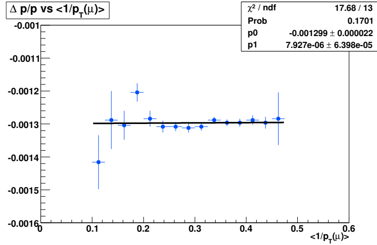
FIGURE 8.18: Fitted \Delta p/p as a function of \langle 1/p_T^\mu \rangle , fitted to a straight line.
