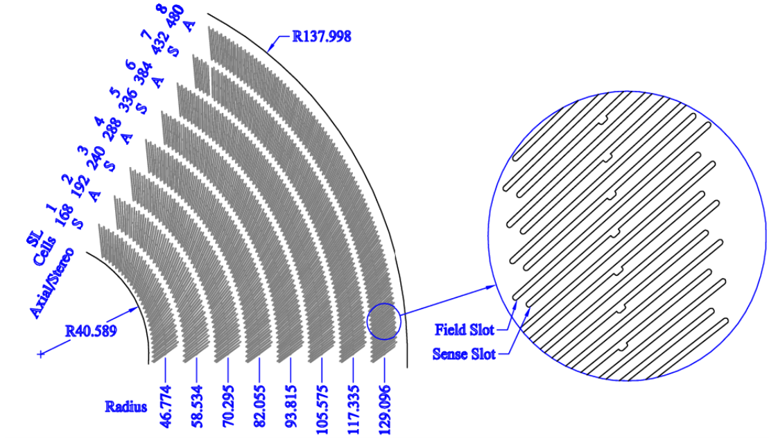
FIGURE 3.5: A view of 1/6 section of the COT.
