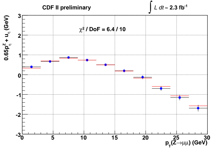
FIGURE 10.4: Mean variation of 0.65 \cdot p_T^\eta(Z) + u_T^\eta as a function of p_T^{Z \rightarrow \mu\mu} using Z \rightarrow \mu\mu events. This plot, together with the corresponding plot using Z \rightarrow ee events, is used in tuning recoil scale parameters. The red histograms are from DukeSim while the blue points are from data. The factor of 0.65 is chosen such that the mean value of 0.65 p_T^\eta(Z) + u_T^\eta is approximately 0.
